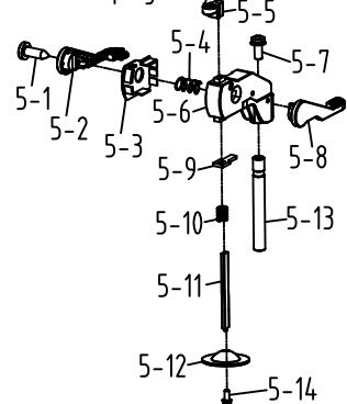
5. Work Clamping assy
